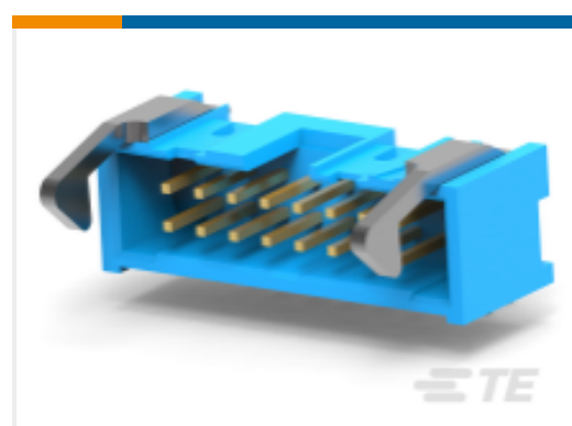
TE Part # 2-1761609-6 IDC LOW PRO HDR 16P RA SHT LAT
